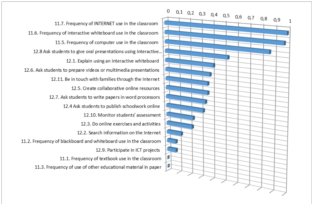
Figure 2. Relative significance of every predictor in clusters' configuration
